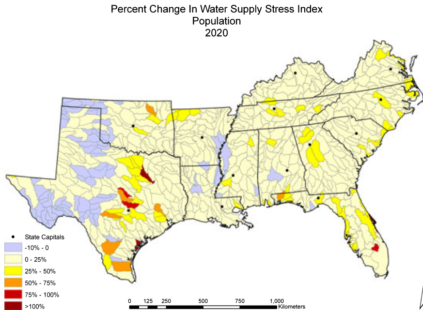
FIGURE 9. Modeled Impact of Population Growth on Water Supply Stress Index (WSSI) Showing Minor Changes in Water Stress Across the Southern U.S. in 2020.
