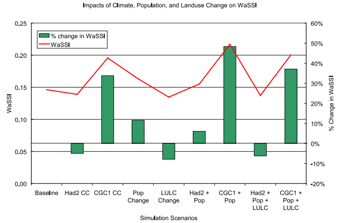
FIGURE 7. Overall Impacts of Climate Change, Land Use Change, Population Change on Water Supply Stress Index (WaSSI = Water Demand/Water Supply) in 2020. Changes in WaSSI are determined by comparing WaSSI in 2020 for each scenario and the baseline WaSSI in 1995.
