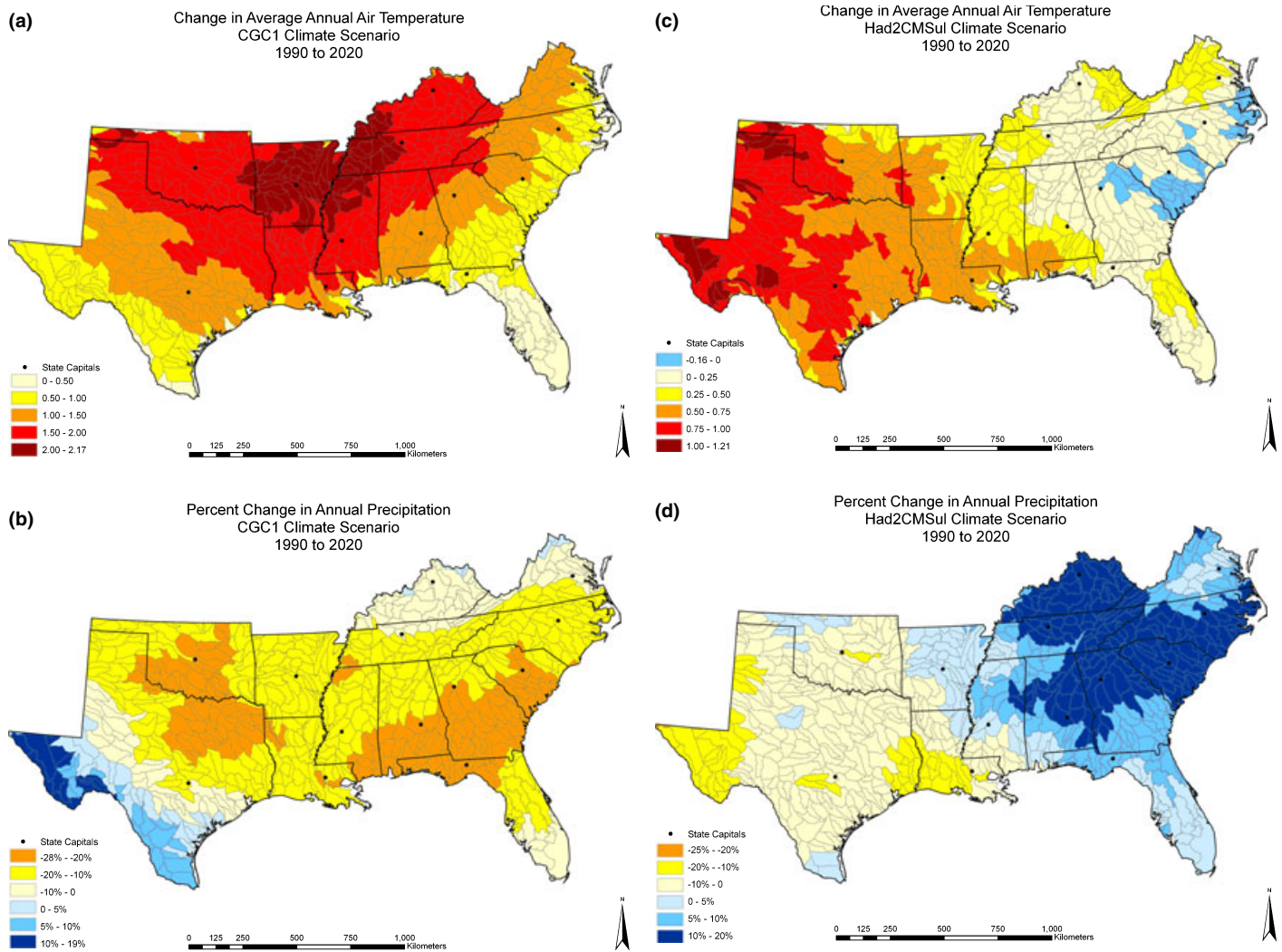
FIGURE 3. Predicted Changes in Air Temperature and Precipitation Across the Southern U.S. by the CGC1 Model (a and b) and the HadCM2Sul (c and d) Model in 2020.
