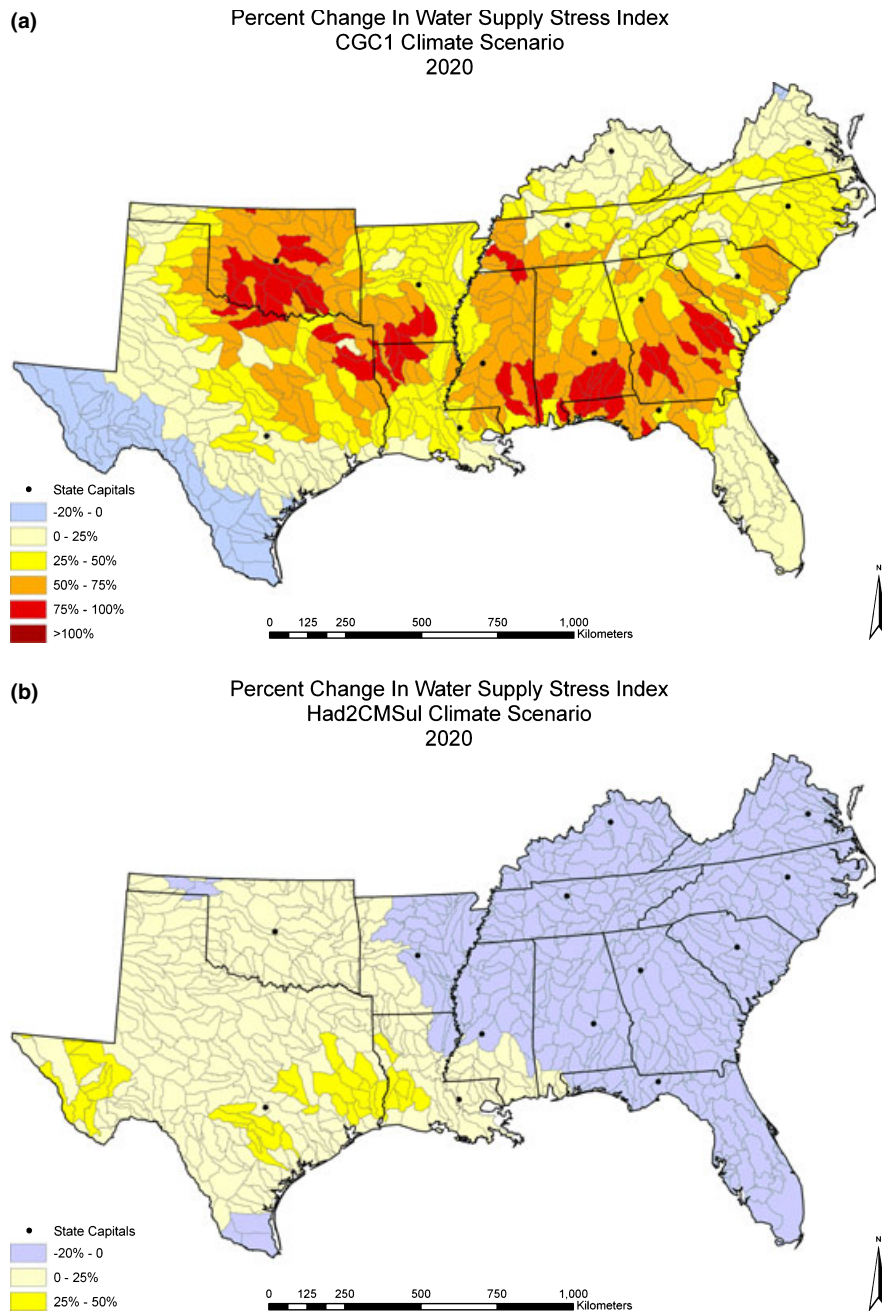
FIGURE 8. Modeled Impact of Climate Change (CGC1) (a) and HadCM2Sul (b) Projections on Water Supply Stress Index (WSSI) Showing Distinct Trends in Water Stress Across the Southern U.S. in 2020.
