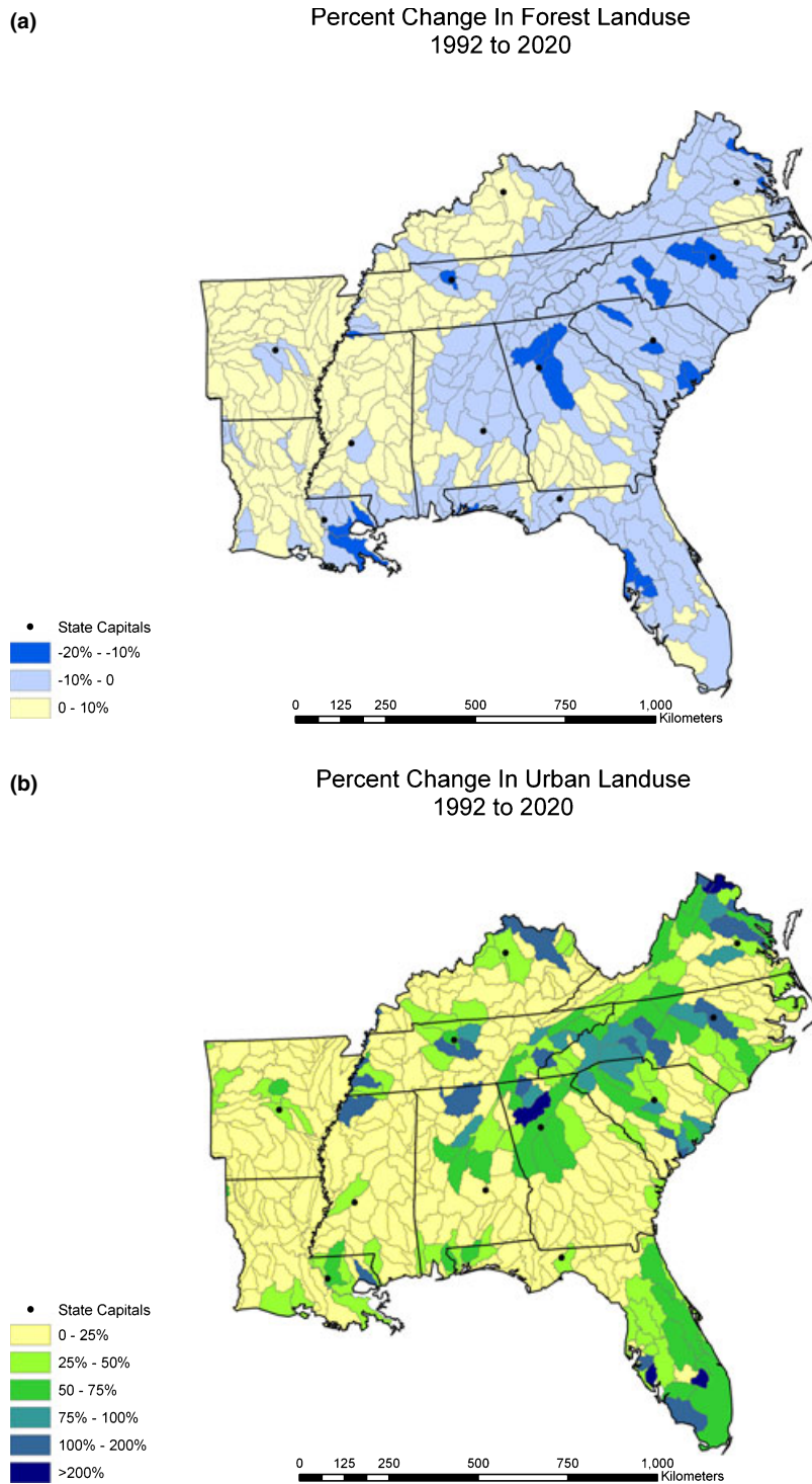
FIGURE 5. Projected Land Use Changes in Forest (a) and Urban (b) Lands in the Southern U.S. by 2020 Showing a Large Increase in Urban Lands in the Piedmont Physiographic Region and Florida.
