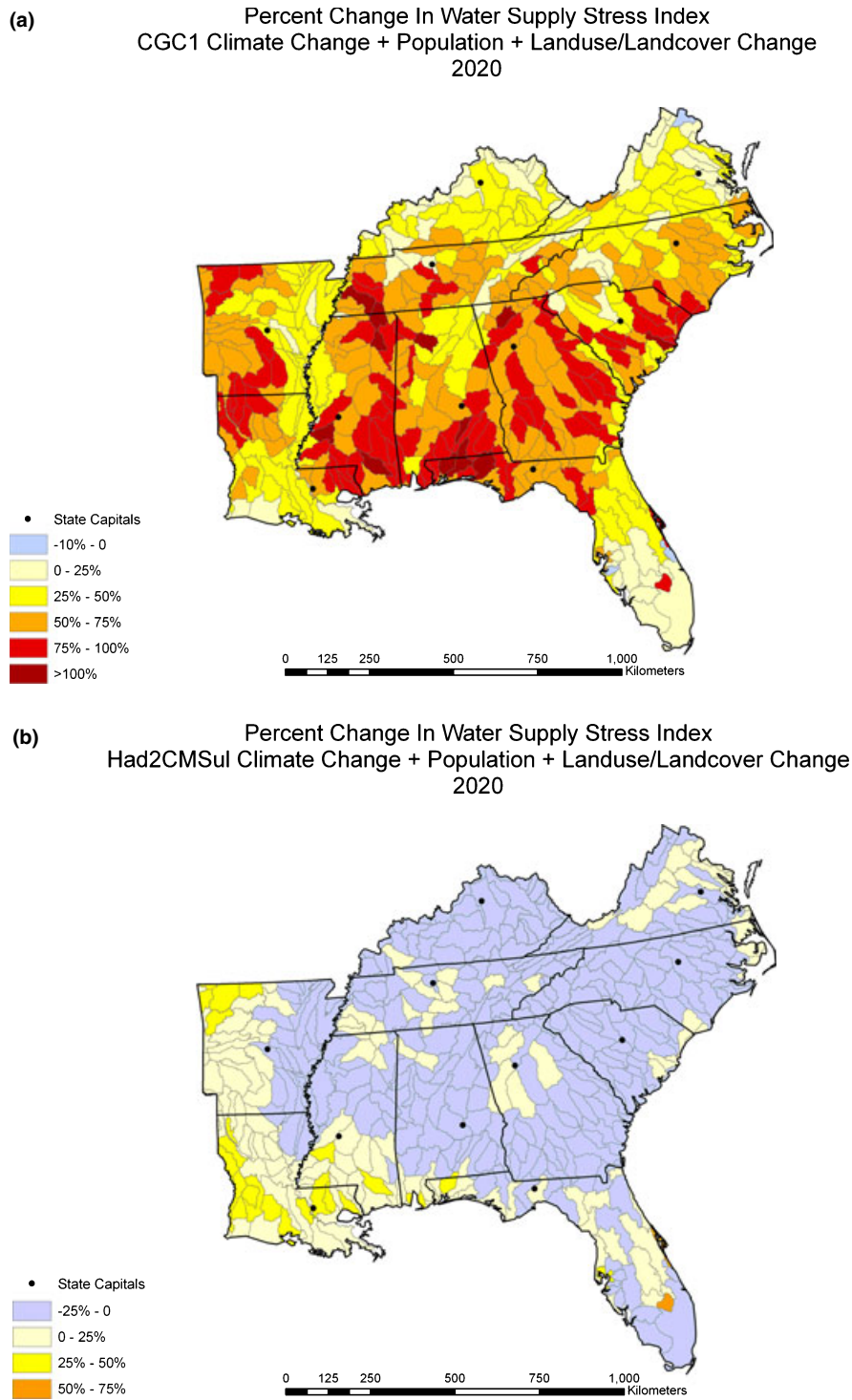
FIGURE 12. Combined Impacts of Future Changes in Climate CGC1 (a) and HadCM2Sul (b), Population, and Land Use (Scenario 6) on Water Supply Stress Index. Two climate change scenarios resulted in distinct water stress trend in 2020.
