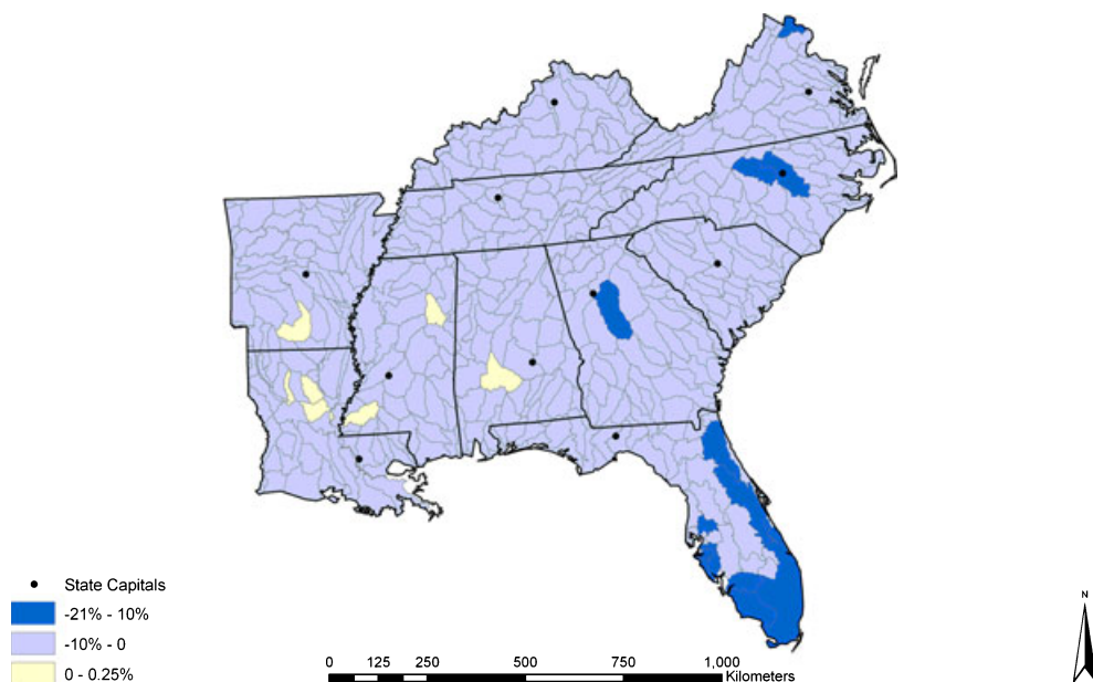
FIGURE 10. Modeled Impact of Land Use Change on Water Supply Stress Index (WSSI) Showing Minor Changes in Water Stress Across the Southern U.S. in 2020.
