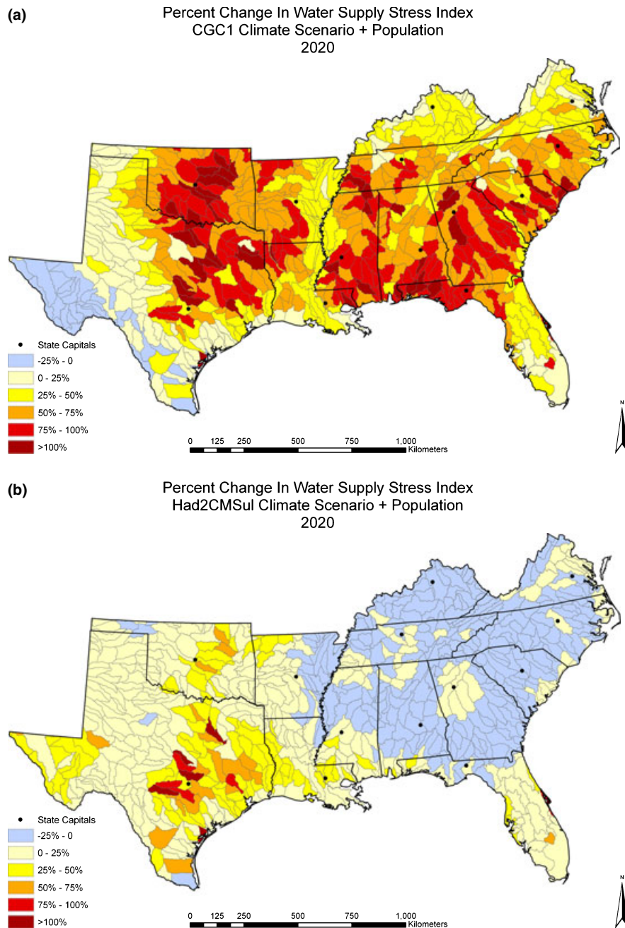
FIGURE 11. Combined Impact of Future Changes in Climate (CGC1) (a) and HadCM2Sul (b) and Population Growth (Scenario 5) on Water Supply Stress Index Showing Increased Water Stress Dominated by Climate Change in 2020.
